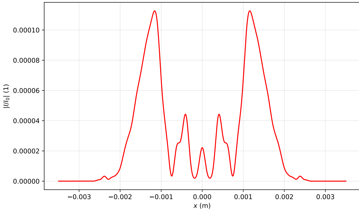
Intensity profile I(x, y = 0, z = 2.627)/I_0 , P_{in}=9.0P_{cr} , artificial time
